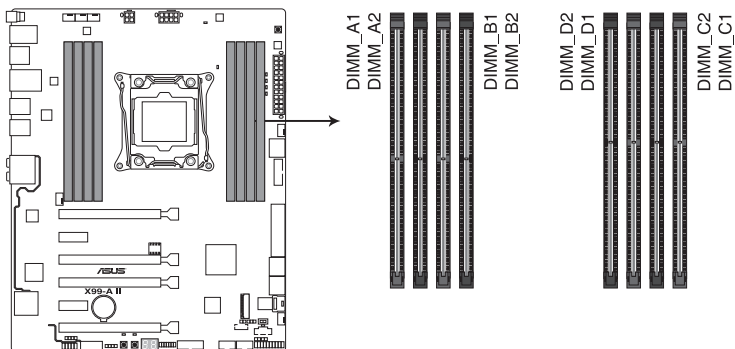
X99-A II 288-pin DDR4 DIMM socket
